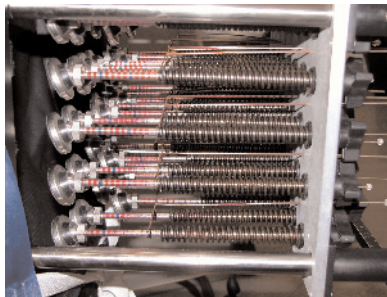
Figure 2: Side view of thirty-five spring-loaded diodes.
